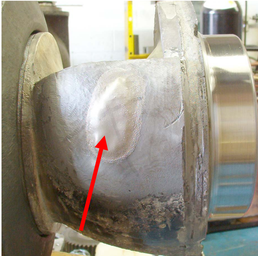
Cast Iron Impeller Weld Repair
